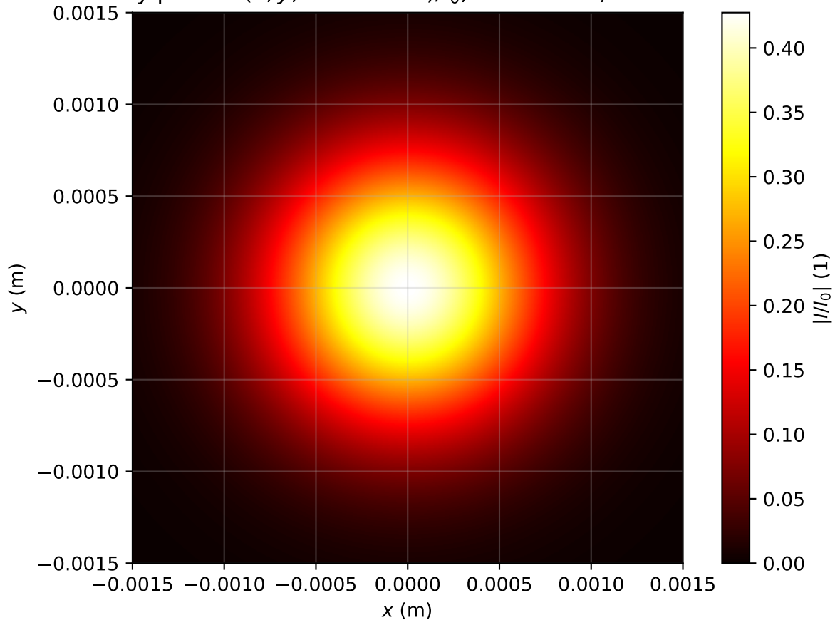
Intensity profile I(x, y, z = 2.707m)/I_0 , P_{in}=0.2P_{cr} , artificial time
